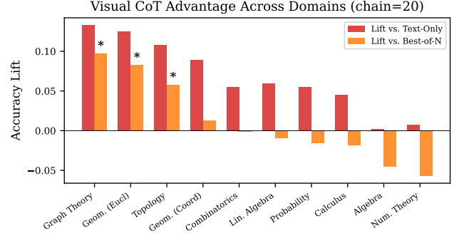
Figure 4: Visual CoT accuracy lift across domains at chain length 20. Red bars: lift over text-only. Orange bars: lift over compute-matched best-of-N. Asterisks mark conditions where 95% CIs do not overlap.
