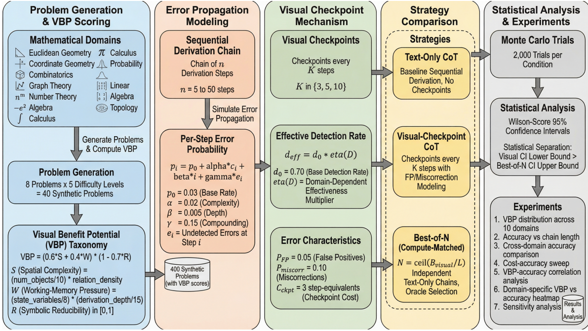
Figure 1: Simulation framework for investigating multimodal interleaved chain-of-thought reasoning in mathematics. The pipeline generates 400 synthetic problems across 10 mathematical domains with Visual Benefit Potential (VBP) scoring, simulates sequential derivation chains with error propagation ( p_i = p_0 + \alpha c_i + \beta i + \gamma e_i ), applies visual checkpoints every K steps with domain-dependent detection rates including false-positive ( P_{FP} = 0.05 ) and miscorrection ( P_{miscorr} = 0.10 ) modeling, and compares three strategies (text-only CoT, visual-checkpoint CoT, compute-matched best-of- N ) via 2,000 Monte Carlo trials with Wilson-score 95% confidence intervals across seven experiments spanning accuracy analysis, cost sweeps, cross-domain comparison, and sensitivity analysis.
